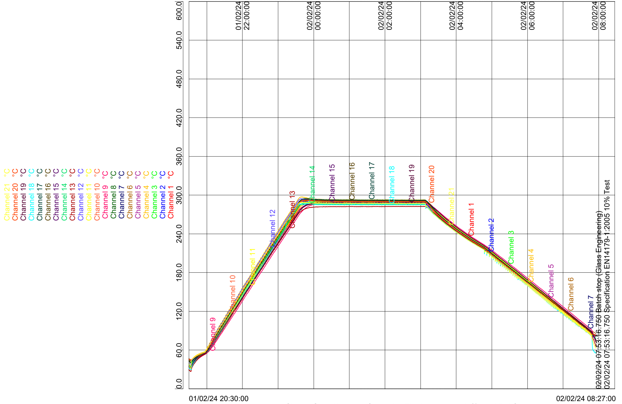
Clayton Glass Heatsoak Calibration EN14179-1-2005 10% Load Full Cycle
